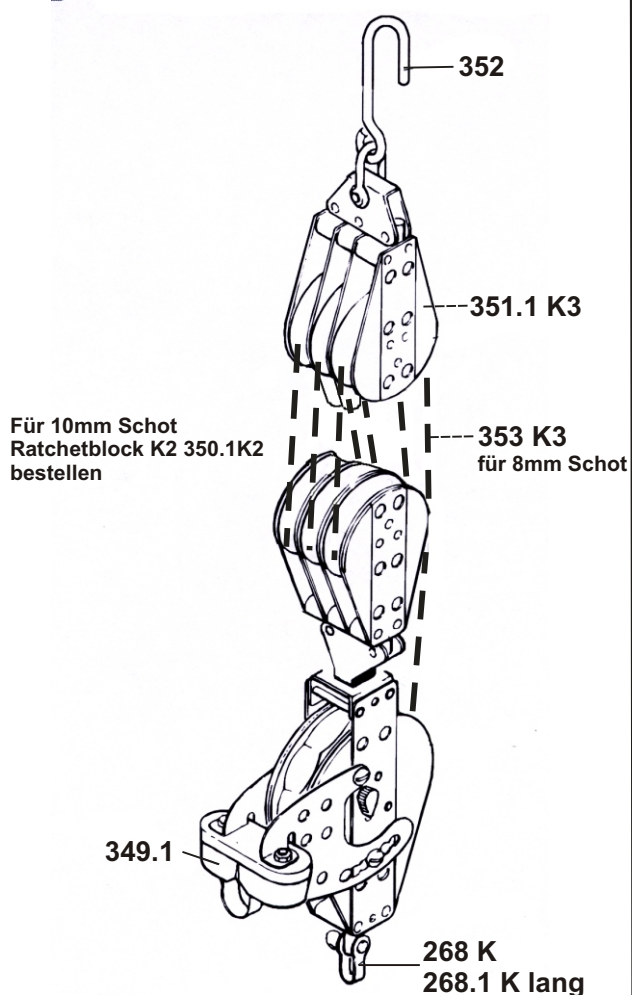
350.1 K3 Ratchetkugellager Block
